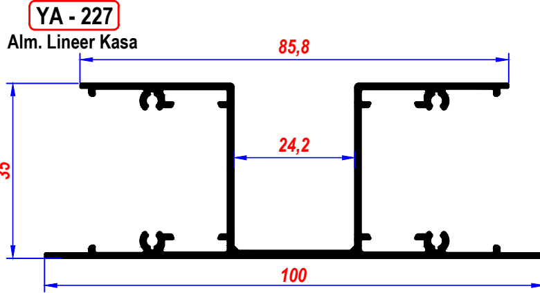
YA-227 ALM.PR.F. 610 cm
