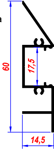
YA-093 Alm.Led Kasa
