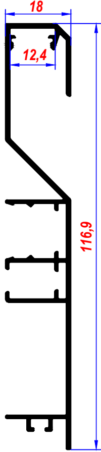
YA-092 ANA KASA PRF.
