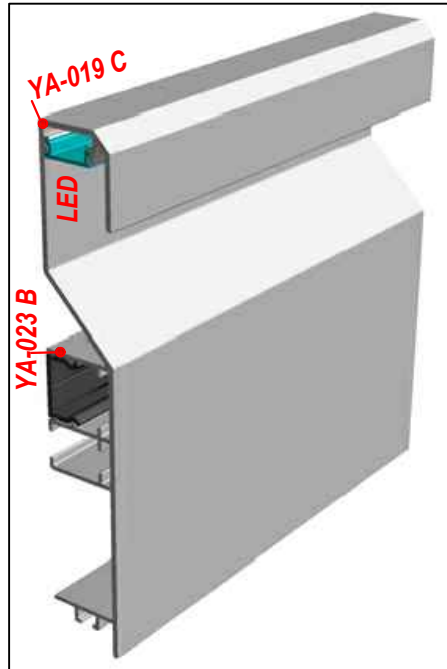
ALM.PRF. - PC. PRF 610 mm
