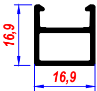
ALM. PRF. 610 cm
